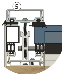
GAVELBALK
